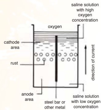
Fig. 3 - Air and oxygen content differentials
