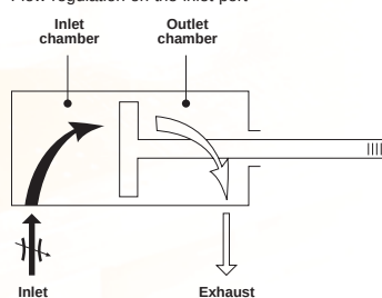
Flow regulation on the inlet port
