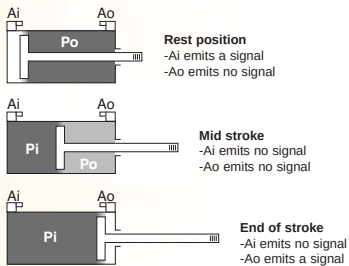
Signals from pressure sensors
