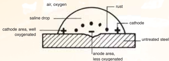
Fig. 4 - Principle of corrosion with different oxygen concentrations.
