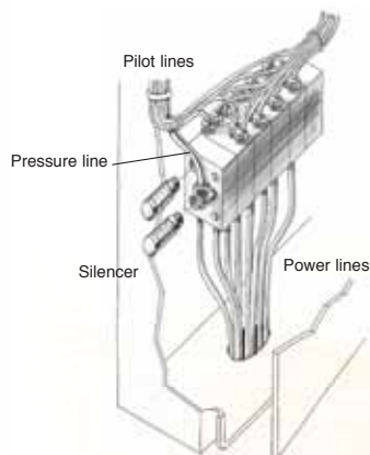
Stackable connection blocks, top and bottom piping
