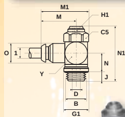
Inlet flow control
