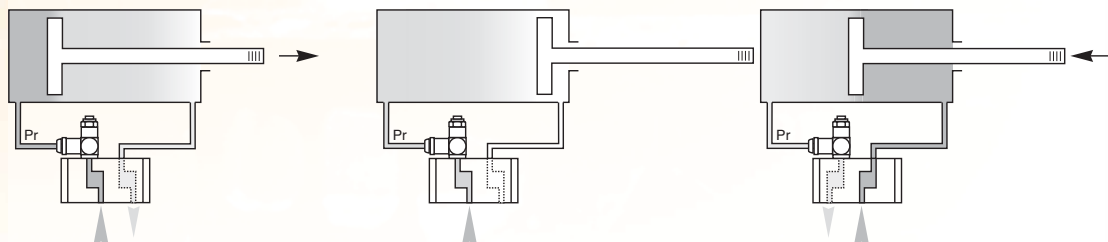
1 - Out stroke
