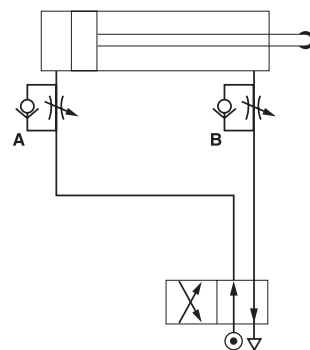
Flow control on a double acting cylinder.
