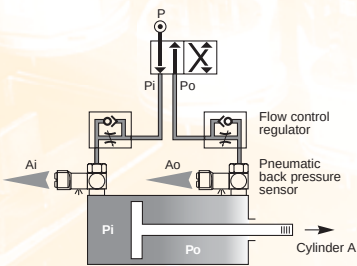
Mounting of pressure sensors
