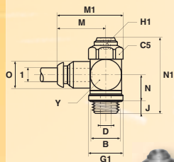
Exhaust flow control
